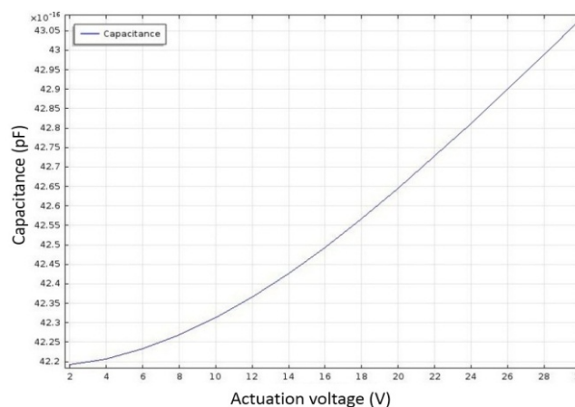
Fig. 8: Capacitance vs. Actuation voltage graph in the comb drive with modified comb fingers
