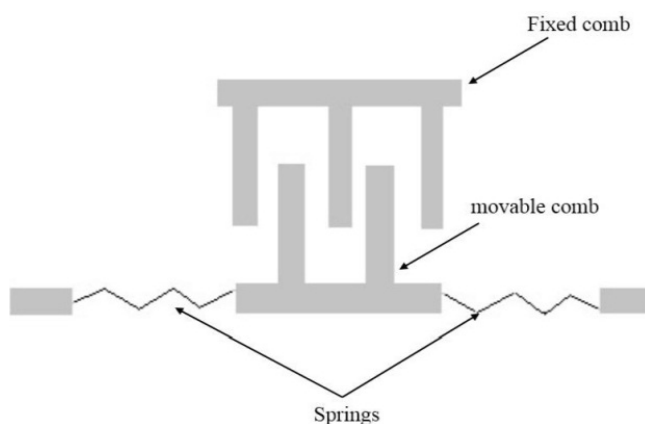
Fig. 1: Basic model of a comb drive.
