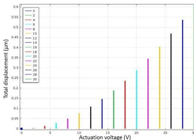
Fig. 7: Displacement vs. Actuation voltage graph in the comb drive with modified comb fingers
